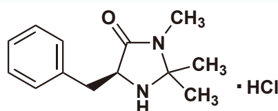
(S)-(-)-5-Benzyl-2,2,3-trimethyl-4-imidazolidinone Hydrochloride
