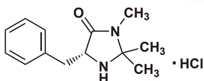
(R)-(+)-5-Benzyl-2,2,3-trimethyl-4-imidazolidinone Hydrochloride
