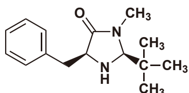
(2S,5S)-(-)-2-tert-Butyl-3-methyl-5-benzyl-4-imidazolidinone
