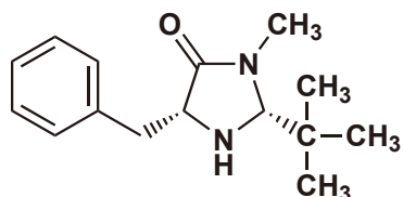
(2R,5R)-(+)-2-tert-Butyl-3-methyl-5-benzyl-4-imidazolidinone
