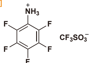
Pentafluoroanilinium Triflate
