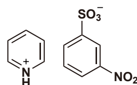
Pyridinium 3-Nitrobenzenesulfonate
