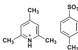
CPTS
