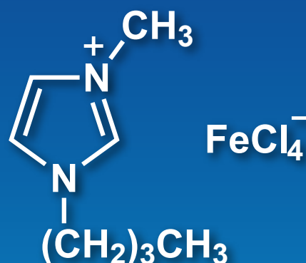
1-Butyl-3-methylimidazolium Tetrachloroferrate
