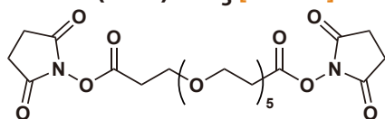
Bis(NHS)PEG 5 [B3728]
