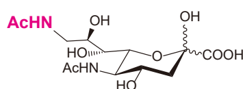
N -Acetyl-9-deoxy-9-acetamidoneuraminic Acid
