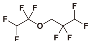
1,1,2,2-Tetrafluoroethyl 2,2,3,3-Tetrafluoropropyl Ether
