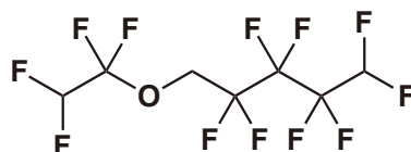
1H,1H,5H-Octafluoropentyl 1,1,2,2-Tetrafluoroethyl Ether
