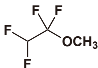
Methyl 1,1,2,2-Tetrafluoroethyl Ether
