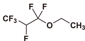
Ethyl 1,1,2,3,3,3-Hexafluoropropyl Ether
