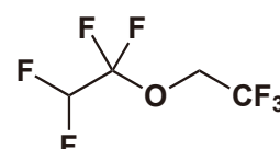
1,1,2,2-Tetrafluoroethyl 2,2,2-Trifluoroethyl Ether
