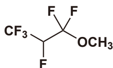
1,1,2,3,3,3-Hexafluoropropyl Methyl Ether
