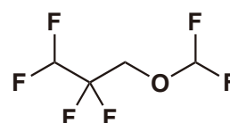
Difluoromethyl 2,2,3,3-Tetrafluoropropyl Ether
