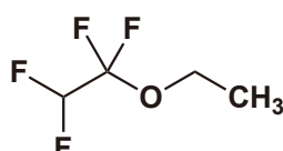
Ethyl 1,1,2,2-Tetrafluoroethyl Ether
